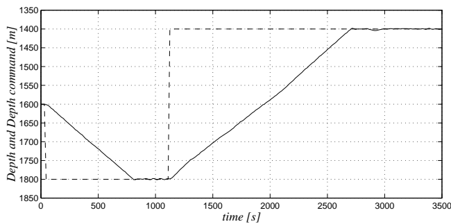
Figure 6: Commanded and measured depth.
