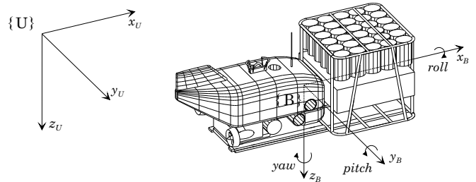
Figure 1: The Sirene coupled to a benthic laboratory. Body-fixed ( \{B\} ) and earth-fixed ( \{U\} ) reference frames.
