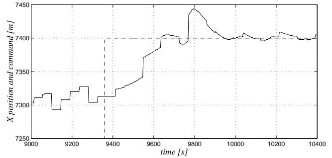
Figure 7: Commanded and measured X position.
