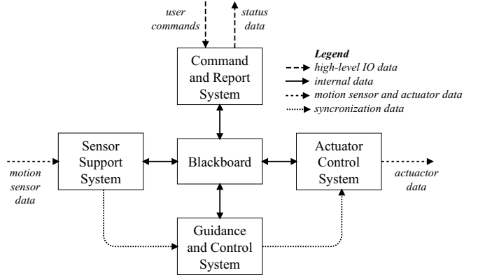
Figure 2: Software system organization and data communication paths.
