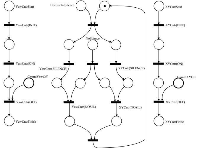
Figure 4: Command of the Yaw and XY controllers in the horizontal plane.
