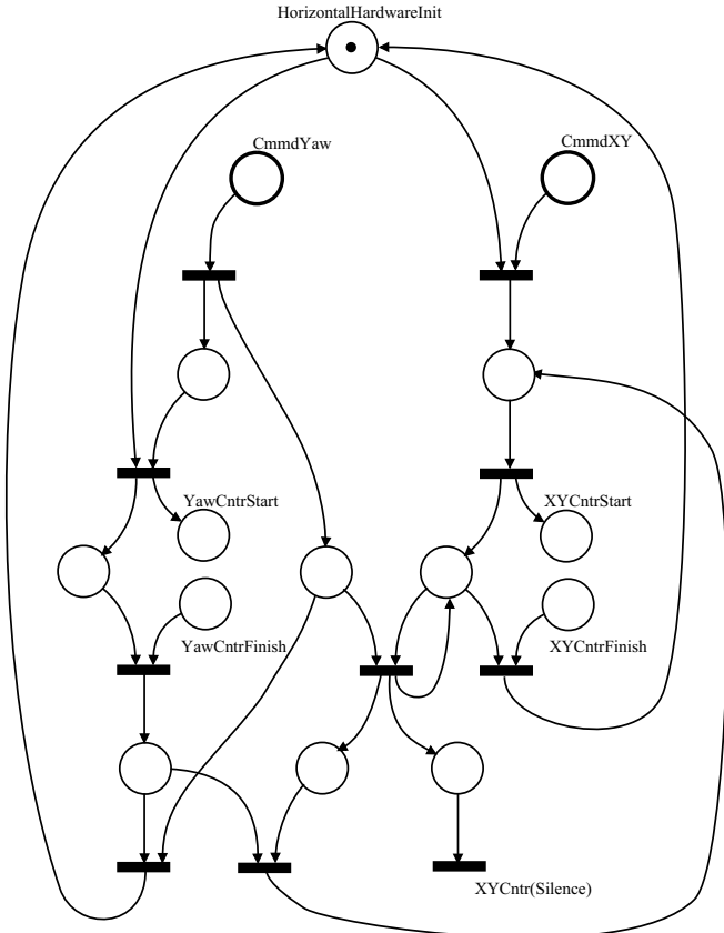
Figure 3: A high-level system synchronization example using Petri Nets
