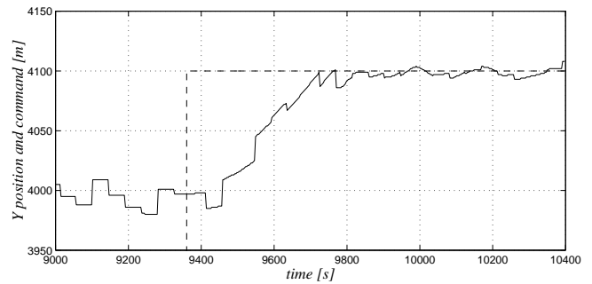
Figure 8: Commanded and measured Y position.
