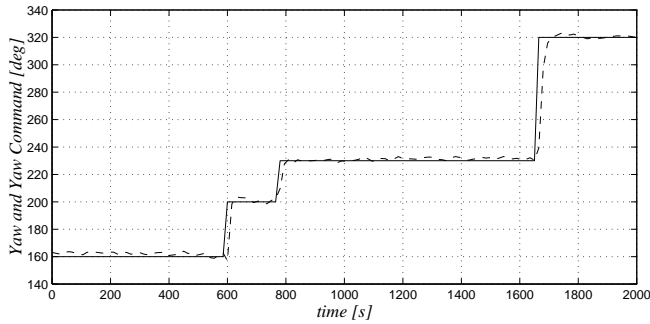
Figure 5: Commanded and measured yaw angle.
