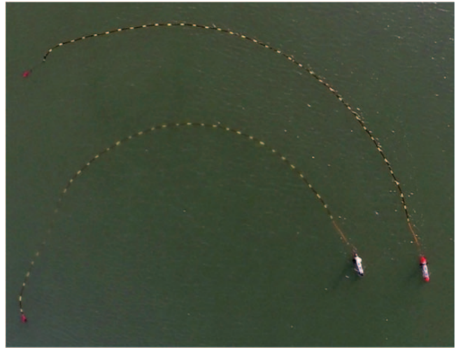
Fig. 3. Aerial view of two MEDUSA vehicles (IST) towing two streamer in a curve.
